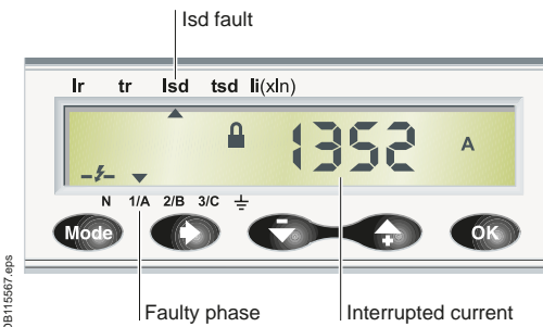
Display of interrupted phase current.
