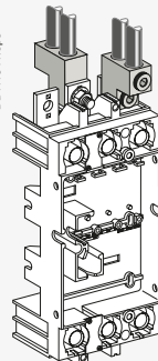
With a 400/630 A base.
